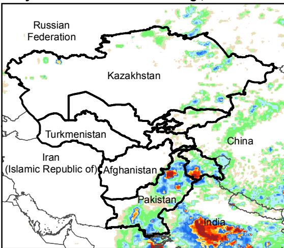
Daily Rainfall estimate for 10 Aug., 2016
