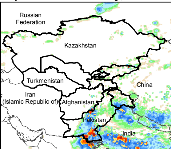
Daily Rainfall estimate for 9 Aug., 2016
