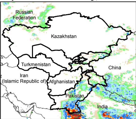
Daily Rainfall estimate for 8 Aug., 2016
