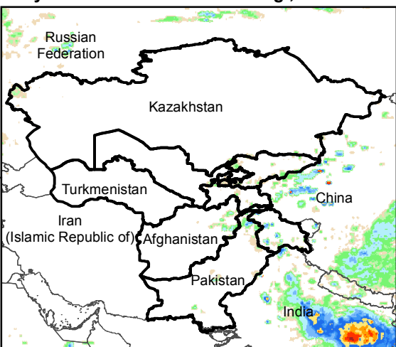
Daily Rainfall estimate for 18 Aug., 2016
