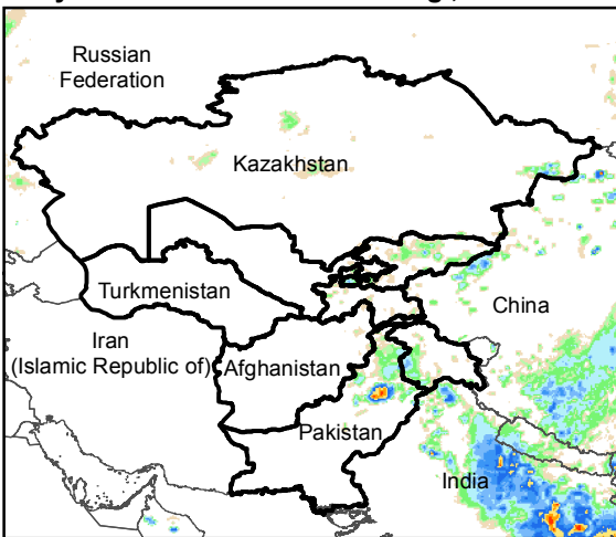
Daily Rainfall estimate for 20 Aug., 2016
