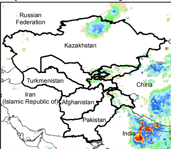
Daily Rainfall estimate for 19 Aug., 2016
