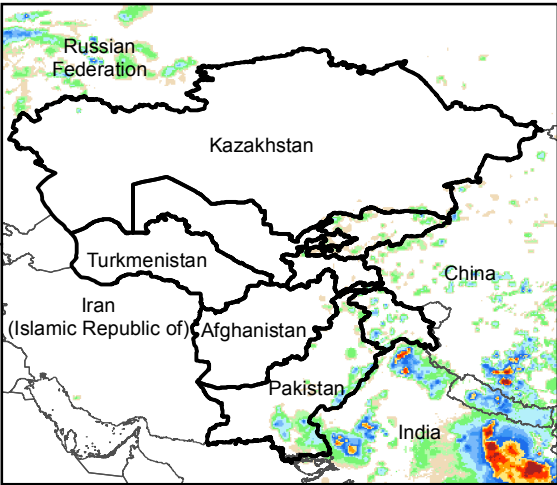
Daily Rainfall estimate for 25 Aug., 2016
