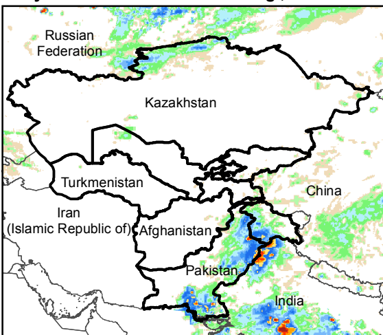
Daily Rainfall estimate for 27 Aug., 2016
