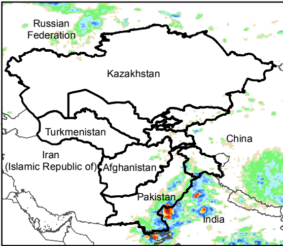
Daily Rainfall estimate for 27 Aug., 2016
