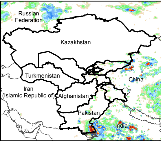
Daily Rainfall estimate for 26 Aug., 2016
