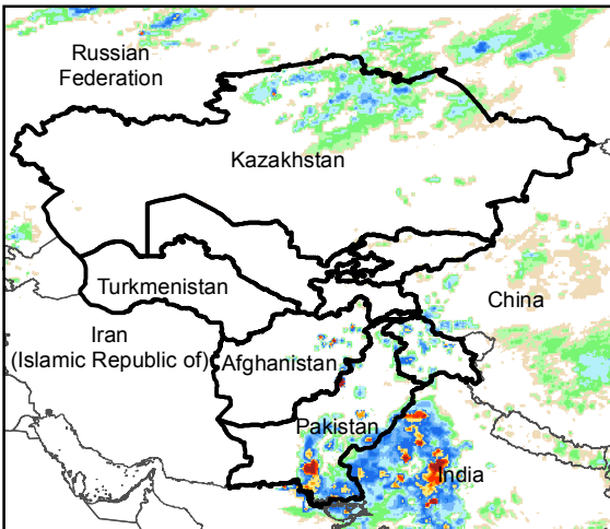
Daily Rainfall estimate for 28 Aug., 2016
