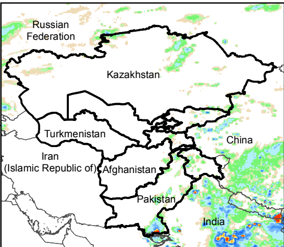
Daily Rainfall estimate for 26 Aug., 2016
