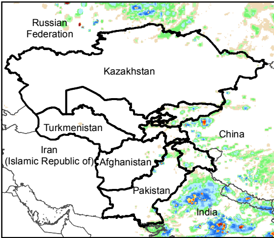
Daily Rainfall estimate for 1 Sep., 2016
