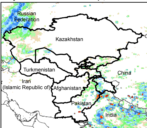
Daily Rainfall estimate for 1 Sep., 2016
