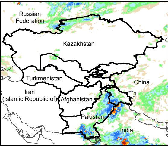
Daily Rainfall estimate for 30 Aug., 2016
