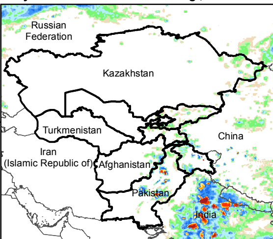
Daily Rainfall estimate for 31 Aug., 2016
