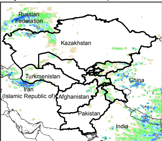
Daily Rainfall estimate for 5 Sep., 2016
