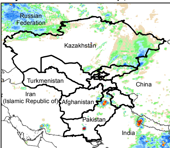
Daily Rainfall estimate for 13 Sep., 2016
