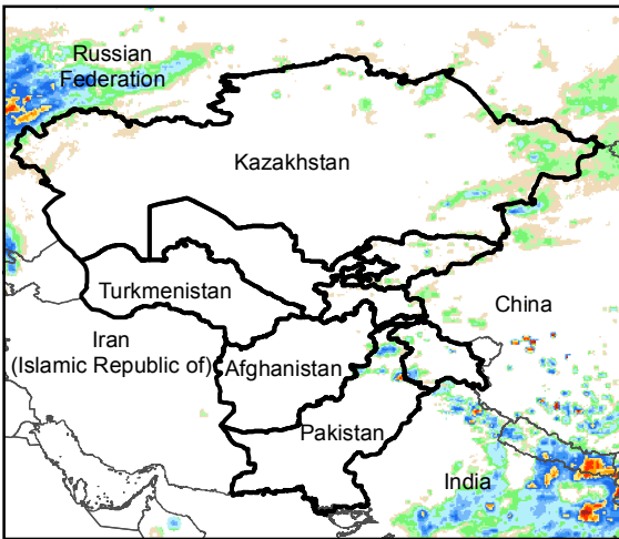
Daily Rainfall estimate for 21 Sep., 2016
