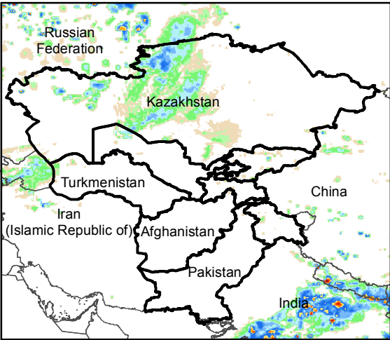
Daily Rainfall estimate for 19 Sep., 2016
