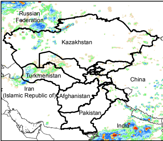
Daily Rainfall estimate for 21 Sep., 2016
