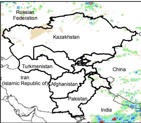
Daily Rainfall estimate for 20 Sep., 2016
