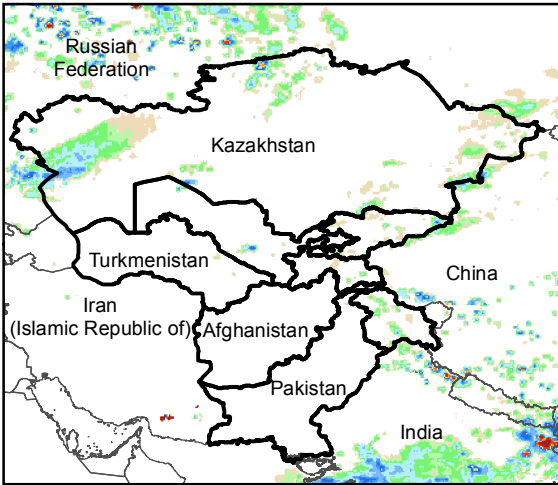
Daily Rainfall estimate for 22 Sep., 2016
