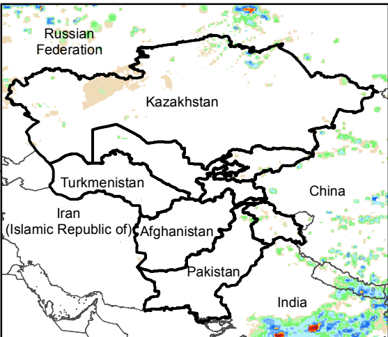
Daily Rainfall estimate for 20 Sep., 2016
