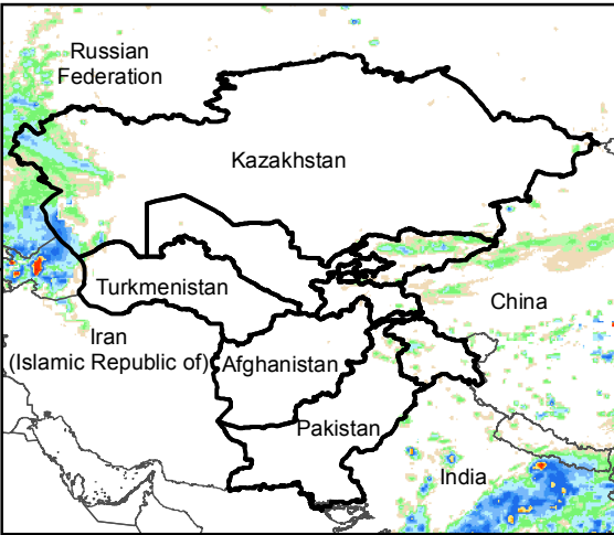
Daily Rainfall estimate for 27 Sep., 2016
