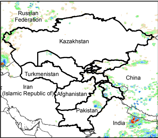
Daily Rainfall estimate for 26 Sep., 2016
