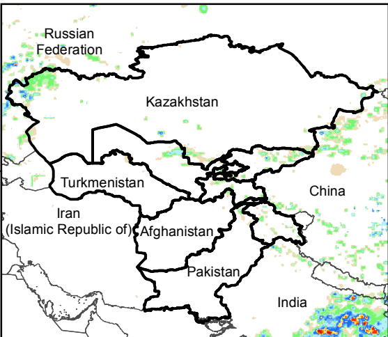
Daily Rainfall estimate for 26 Sep., 2016
