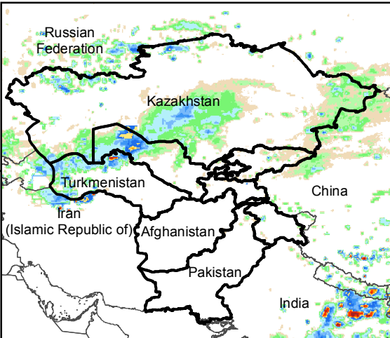
Daily Rainfall estimate for 29 Sep., 2016
