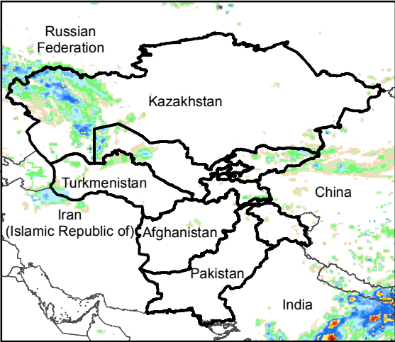
Daily Rainfall estimate for 28 Sep., 2016
