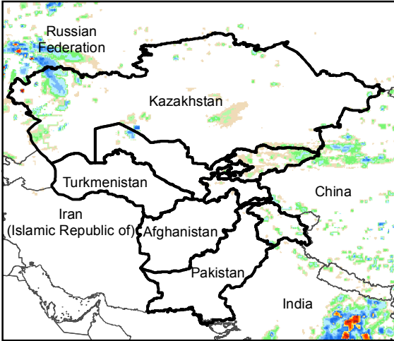
Daily Rainfall estimate for 30 Sep., 2016
