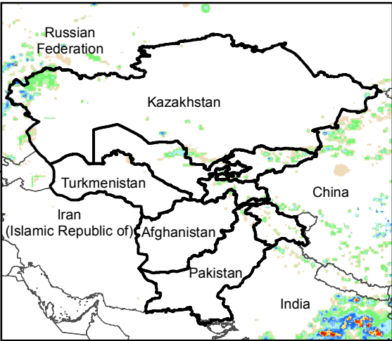
Daily Rainfall estimate for 29 Sep., 2016
