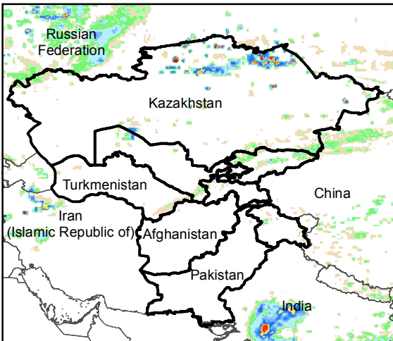
Daily Rainfall estimate for 1 Oct., 2016
