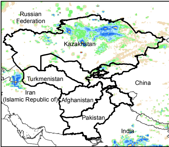
Daily Rainfall estimate for 3 Oct., 2016
