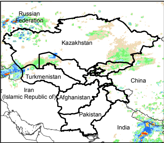
Daily Rainfall estimate for 1 Oct., 2016
