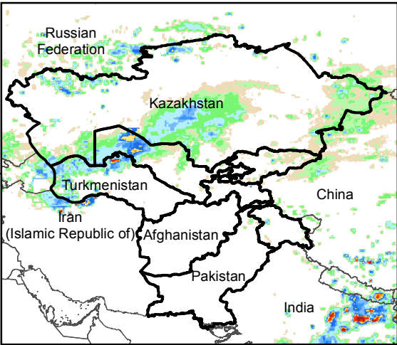
Daily Rainfall estimate for 2 Oct., 2016
