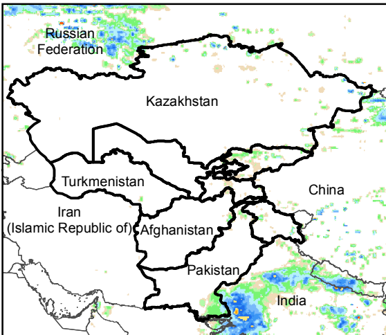
Daily Rainfall estimate for 4 Oct., 2016
