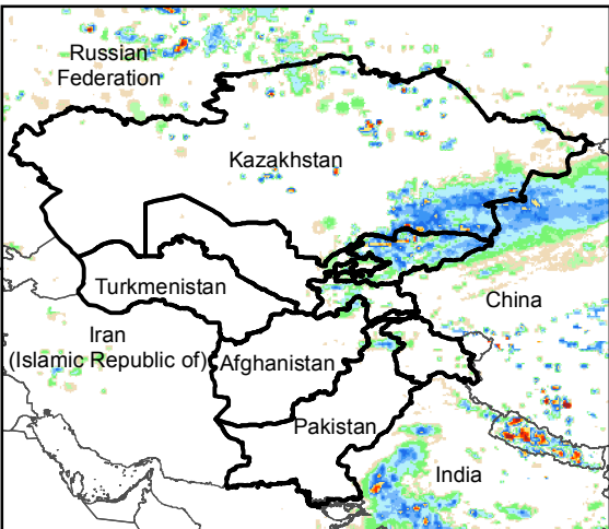
Daily Rainfall estimate for 2 Oct., 2016
