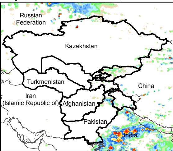
Daily Rainfall estimate for 8 Oct., 2016
