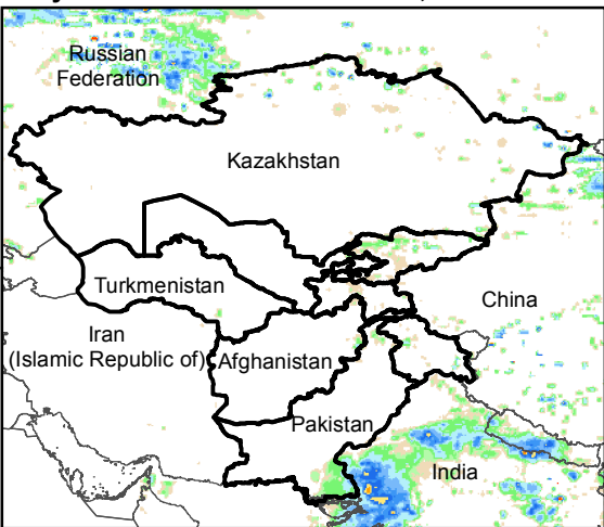
Daily Rainfall estimate for 7 Oct., 2016
