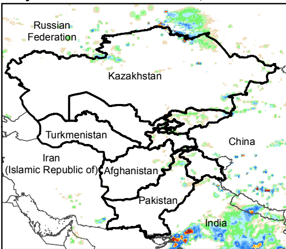
Daily Rainfall estimate for 9 Oct., 2016
