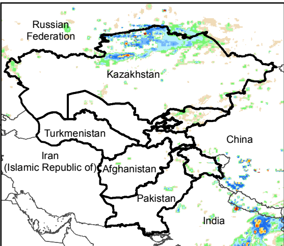
Daily Rainfall estimate for 9 Oct., 2016
