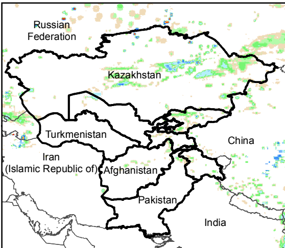
Daily Rainfall estimate for 11 Oct., 2016
