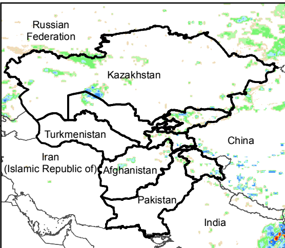
Daily Rainfall estimate for 10 Oct., 2016
