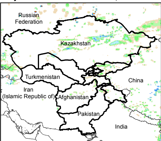
Daily Rainfall estimate for 11 Oct., 2016
