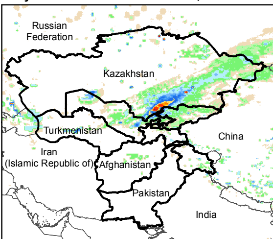
Daily Rainfall estimate for 13 Oct., 2016
