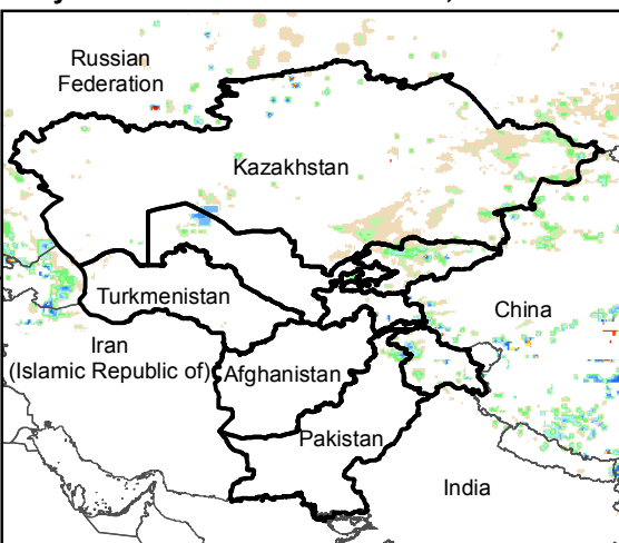
Daily Rainfall estimate for 12 Oct., 2016
