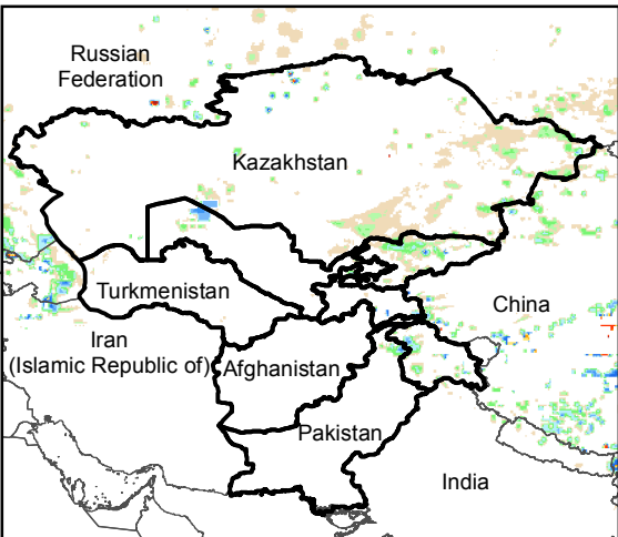
Daily Rainfall estimate for 12 Oct., 2016
