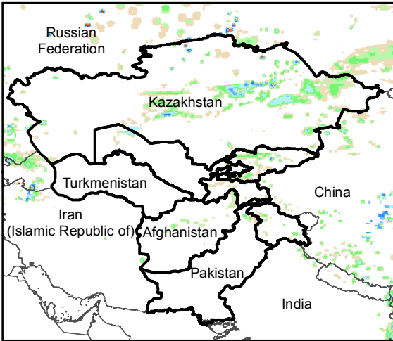
Daily Rainfall estimate for 14 Oct., 2016
