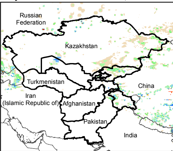
Daily Rainfall estimate for 15 Oct., 2016
