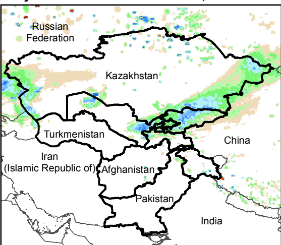
Daily Rainfall estimate for 14 Oct., 2016
