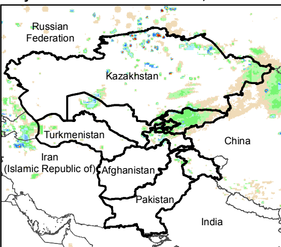
Daily Rainfall estimate for 19 Oct., 2016
