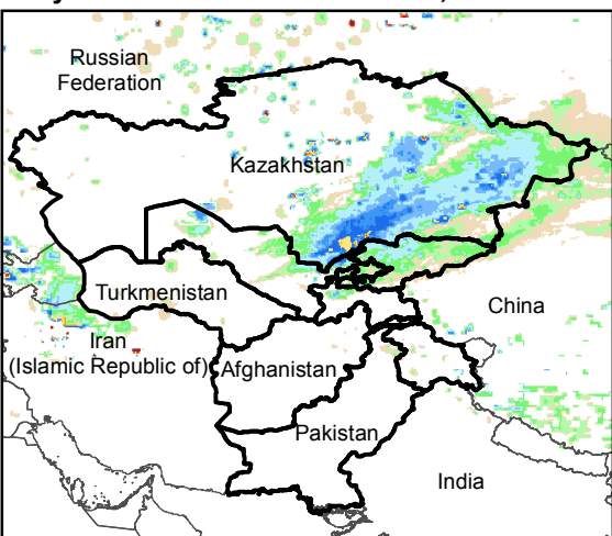
Daily Rainfall estimate for 18 Oct., 2016
