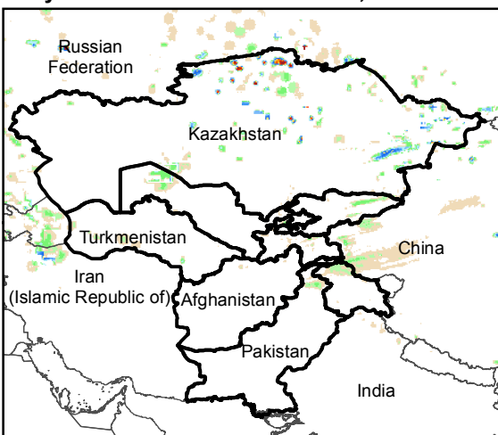
Daily Rainfall estimate for 20 Oct., 2016
