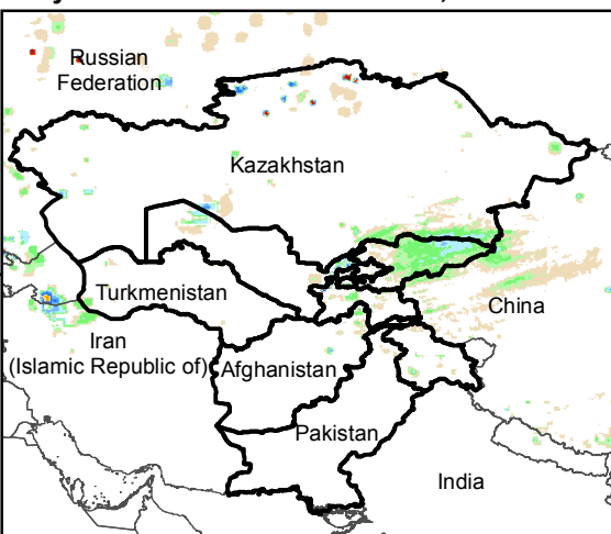
Daily Rainfall estimate for 22 Oct., 2016
