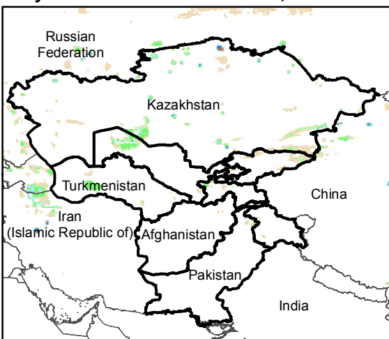
Daily Rainfall estimate for 23 Oct., 2016
