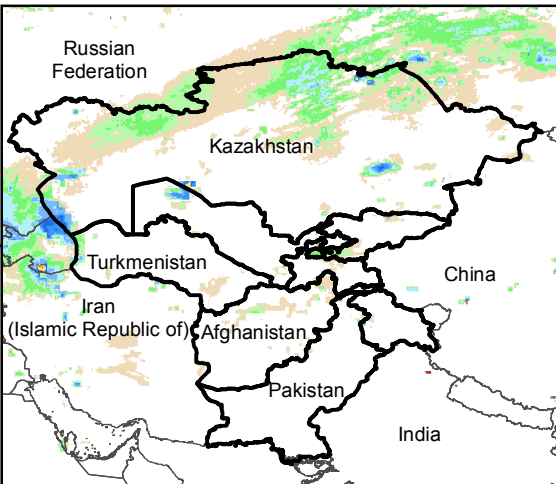
Daily Rainfall estimate for 14 Dec., 2016
