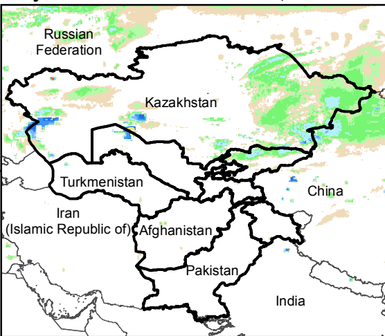
Daily Rainfall estimate for 2 Jan., 2017
