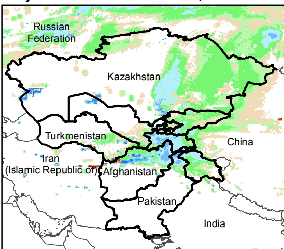
Daily Rainfall estimate for 3 Jan., 2017
