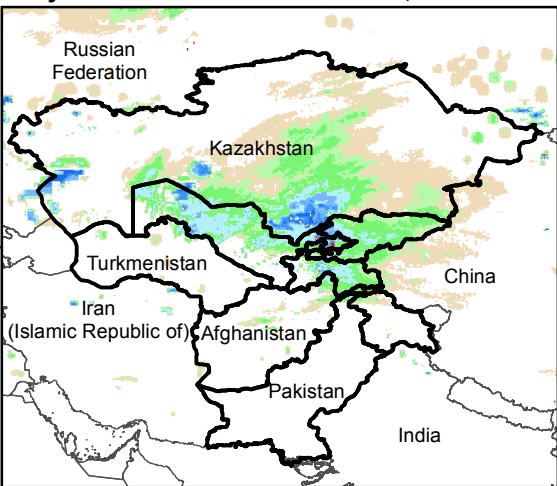
Daily Rainfall estimate for 1 Jan., 2017
