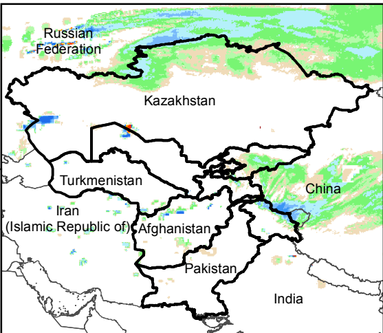
Daily Rainfall estimate for 8 Jan., 2017
