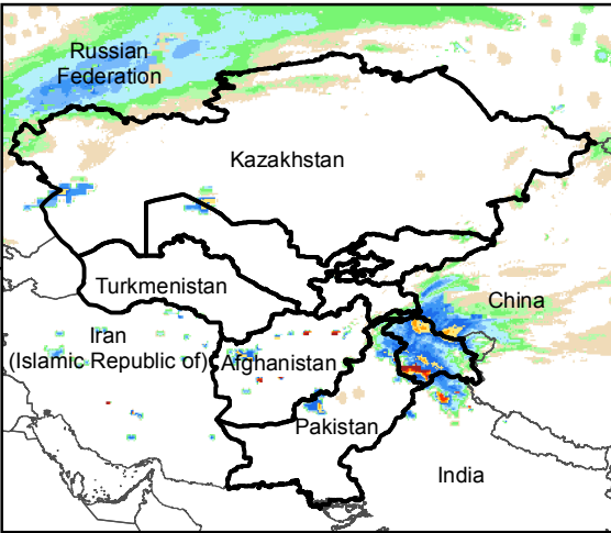
Daily Rainfall estimate for 9 Jan., 2017
