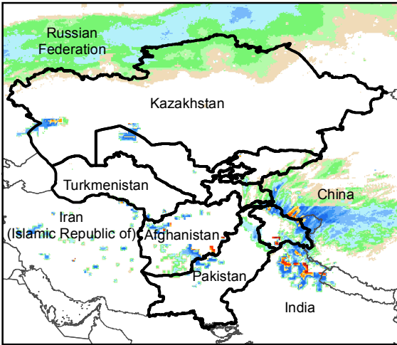
Daily Rainfall estimate for 10 Jan., 2017
