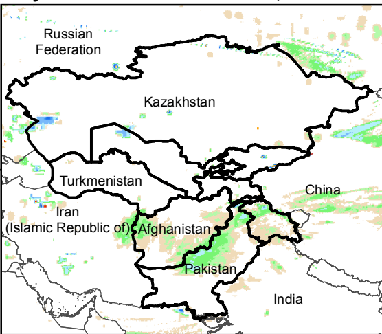
Daily Rainfall estimate for 17 Jan., 2017
