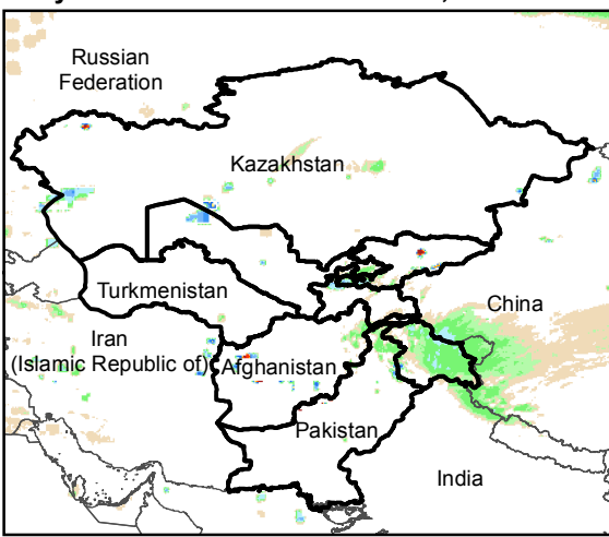
Daily Rainfall estimate for 18 Jan., 2017
