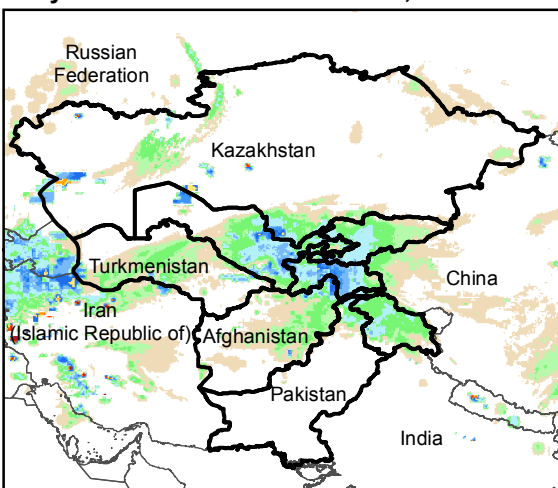
Daily Rainfall estimate for 28 Jan., 2017
