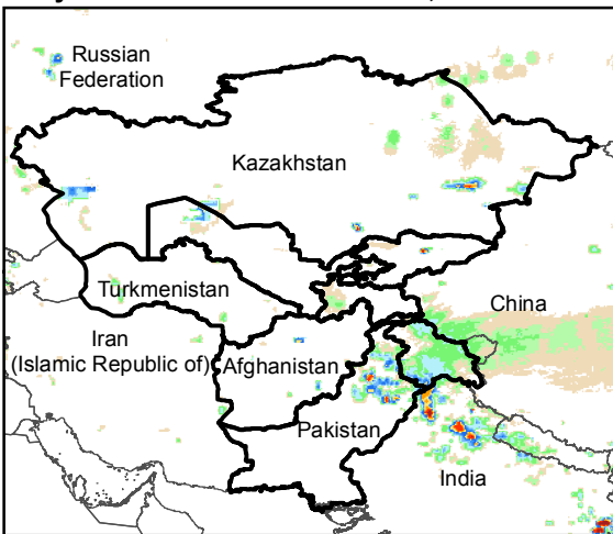
Daily Rainfall estimate for 12 Mar., 2017
