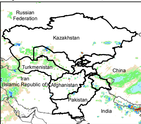
Daily Rainfall estimate for 14 Mar., 2017
