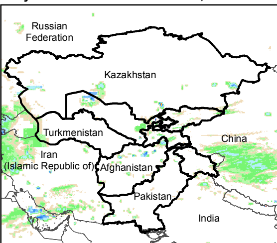
Daily Rainfall estimate for 16 Mar., 2017
