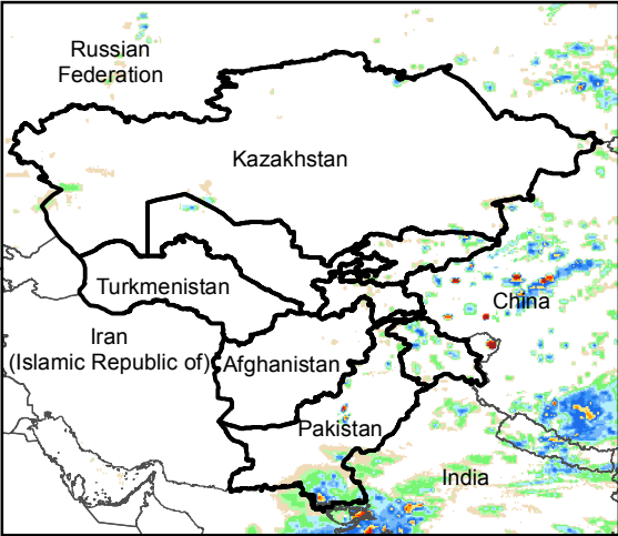
Daily Rainfall estimate for 24 Aug., 2017
