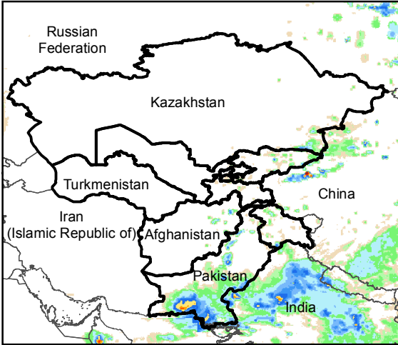
Daily Rainfall estimate for 26 Aug., 2017
