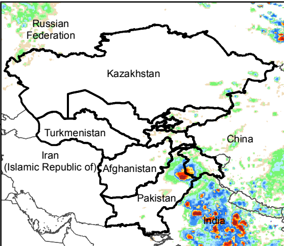
Daily Rainfall estimate for 25 Aug., 2017
