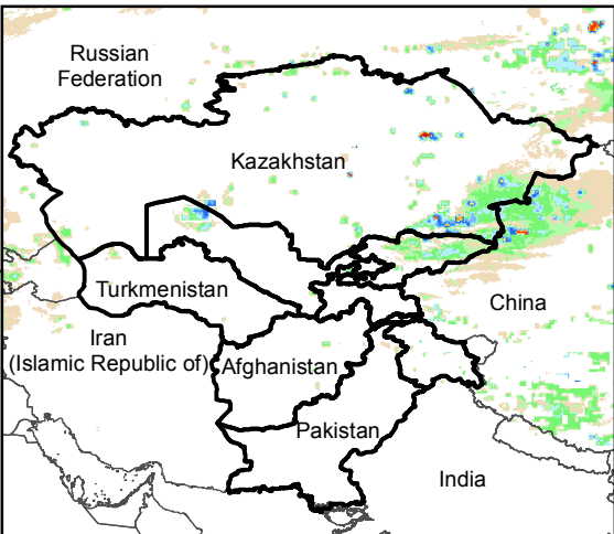
Daily Rainfall estimate for 7 Nov., 2017
