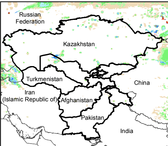
Daily Rainfall estimate for 8 Nov., 2017
