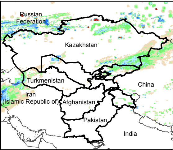
Daily Rainfall estimate for 7 Nov., 2017
