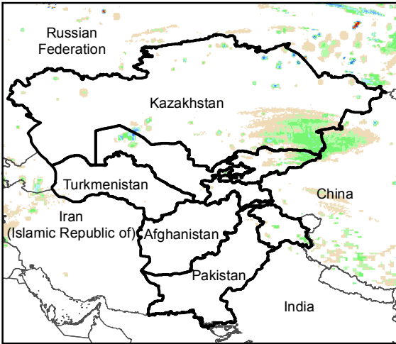
Daily Rainfall estimate for 9 Nov., 2017
