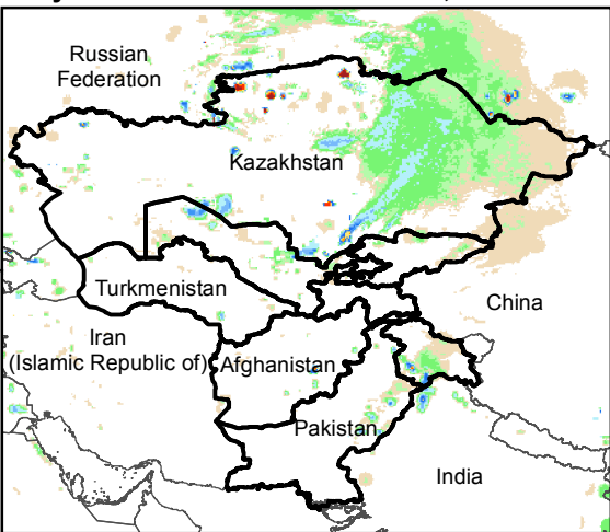
Daily Rainfall estimate for 13 Dec., 2017
