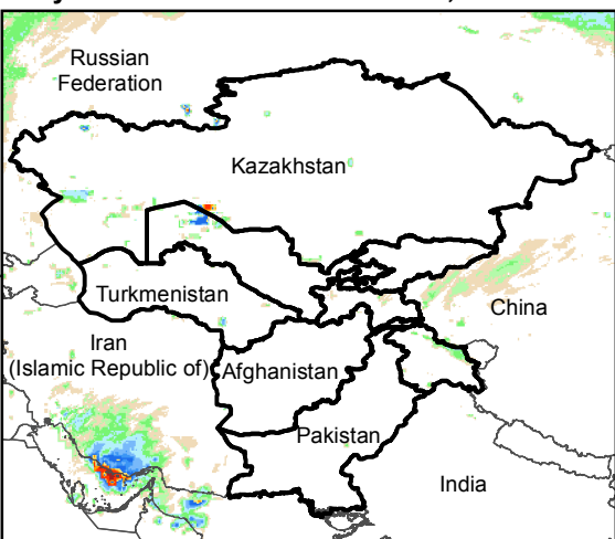
Daily Rainfall estimate for 16 Dec., 2017
