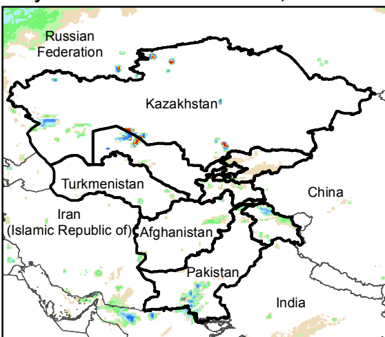
Daily Rainfall estimate for 18 Dec., 2017
