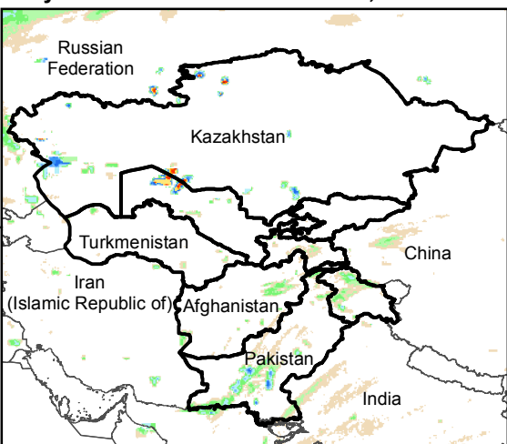
Daily Rainfall estimate for 19 Dec., 2017
