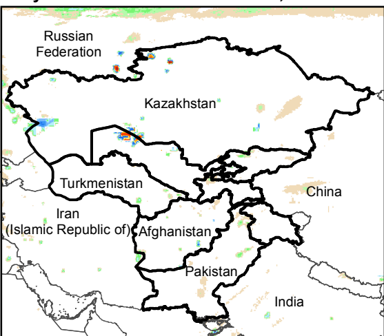
Daily Rainfall estimate for 20 Dec., 2017
