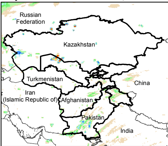
Daily Rainfall estimate for 22 Dec., 2017
