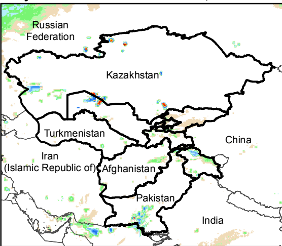
Daily Rainfall estimate for 21 Dec., 2017
