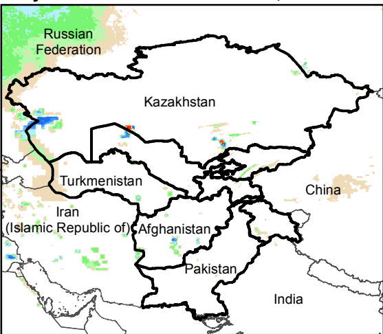
Daily Rainfall estimate for 25 Jan., 2018
