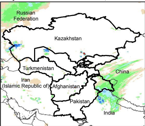
Daily Rainfall estimate for 26 Jan., 2018
