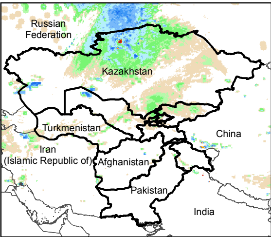
Daily Rainfall estimate for 6 Mar., 2018
