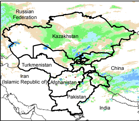
Daily Rainfall estimate for 7 Mar., 2018
