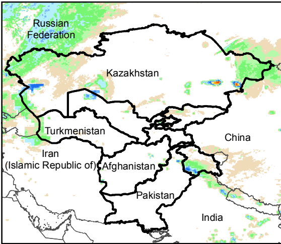
Daily Rainfall estimate for 8 Mar., 2018
