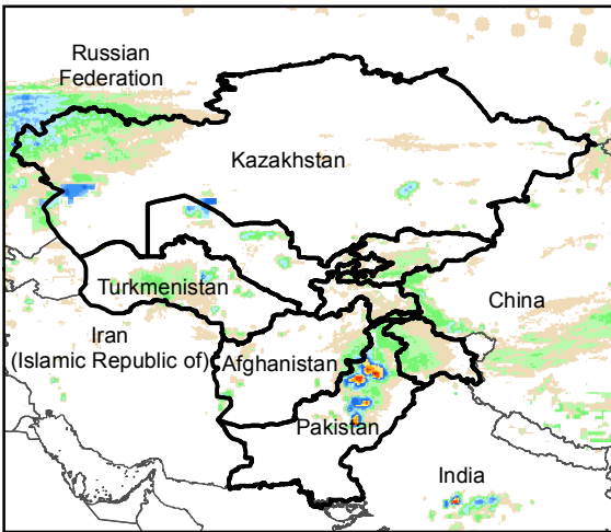
Daily Rainfall estimate for 8 Mar., 2018
