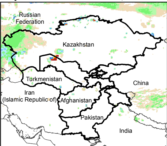
Daily Rainfall estimate for 16 Dec., 2018
