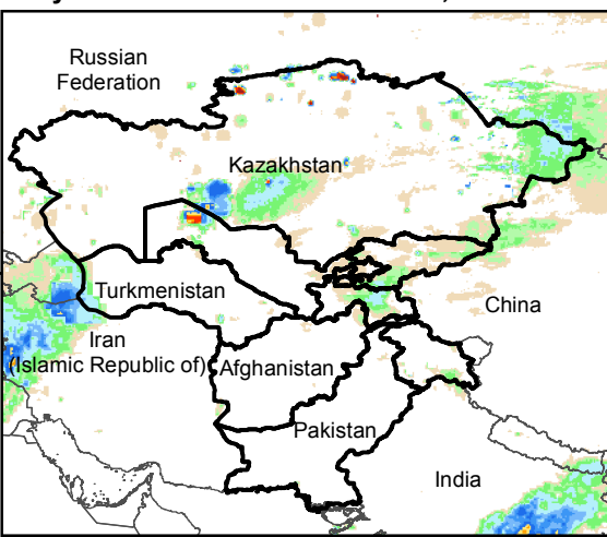
Daily Rainfall estimate for 17 Dec., 2018
