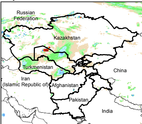
Daily Rainfall estimate for 18 Dec., 2018
