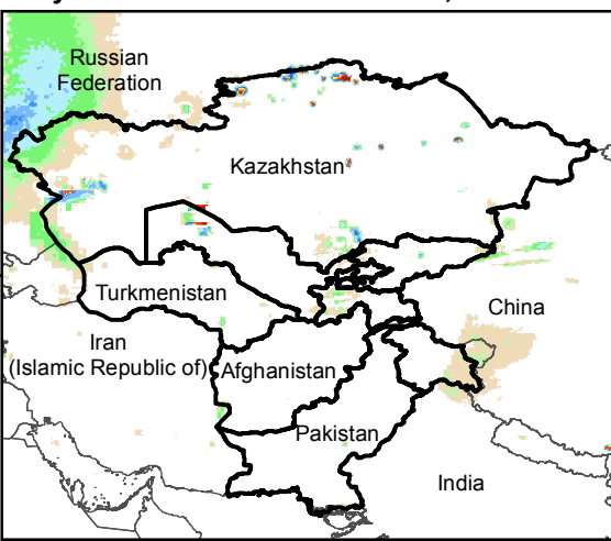
Daily Rainfall estimate for 26 Dec., 2018
