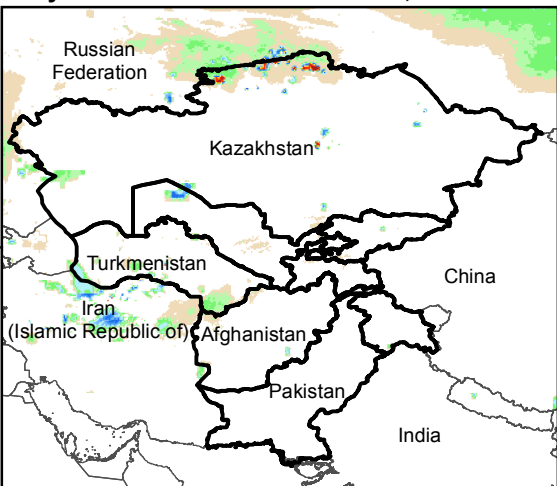
Daily Rainfall estimate for 25 Dec., 2018
