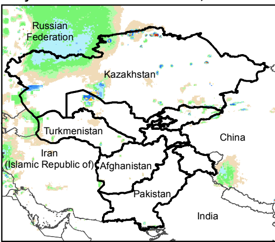
Daily Rainfall estimate for 27 Dec., 2018
