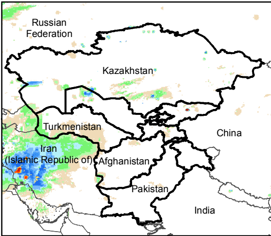
Daily Rainfall estimate for 6 Jan., 2019
