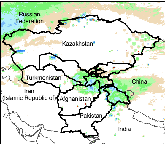
Daily Rainfall estimate for 5 Jan., 2019
