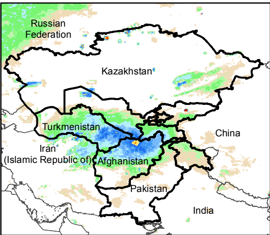
Daily Rainfall estimate for 4 Jan., 2019
