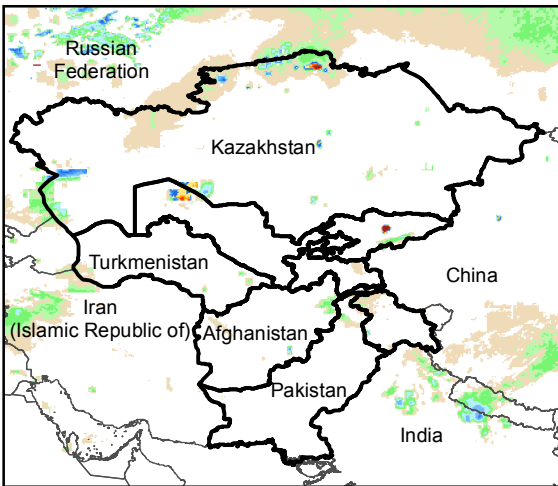
Daily Rainfall estimate for 6 Jan., 2019
