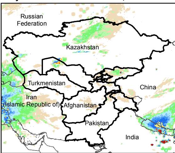
Daily Rainfall estimate for 9 Feb., 2019
