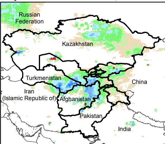
Daily Rainfall estimate for 8 Feb., 2019
