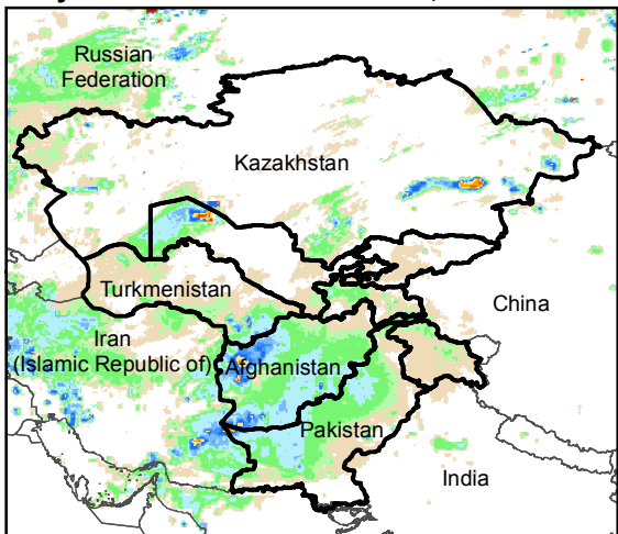
Daily Rainfall estimate for 4 Mar., 2019
