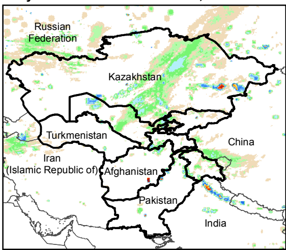
Daily Rainfall estimate for 4 Mar., 2019
