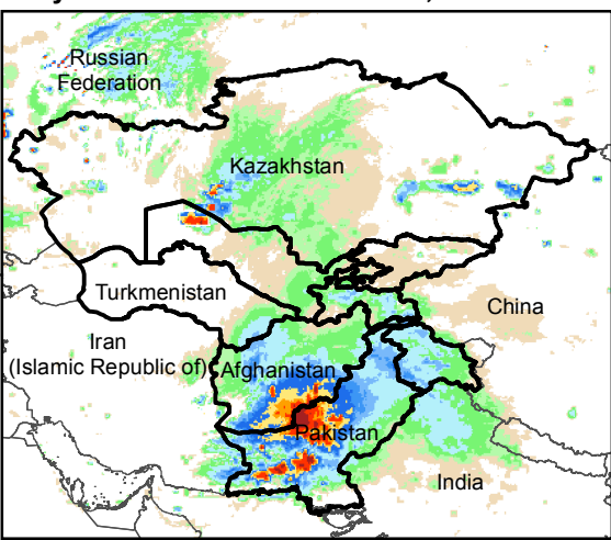
Daily Rainfall estimate for 2 Mar., 2019
