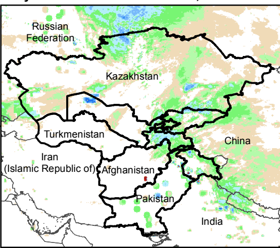
Daily Rainfall estimate for 3 Mar., 2019
