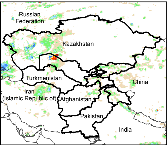
Daily Rainfall estimate for 28 May., 2019
