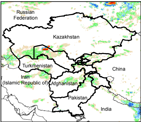
Daily Rainfall estimate for 30 May., 2019
