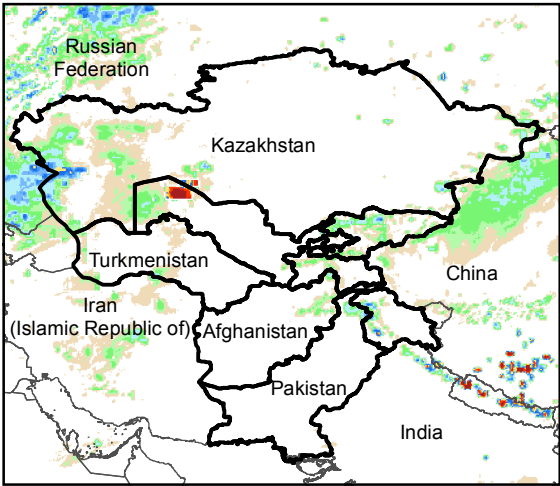
Daily Rainfall estimate for 30 May., 2019
