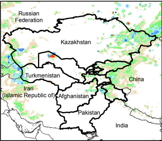
Daily Rainfall estimate for 29 May., 2019
