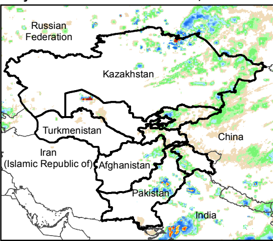
Daily Rainfall estimate for 18 Jun., 2019
