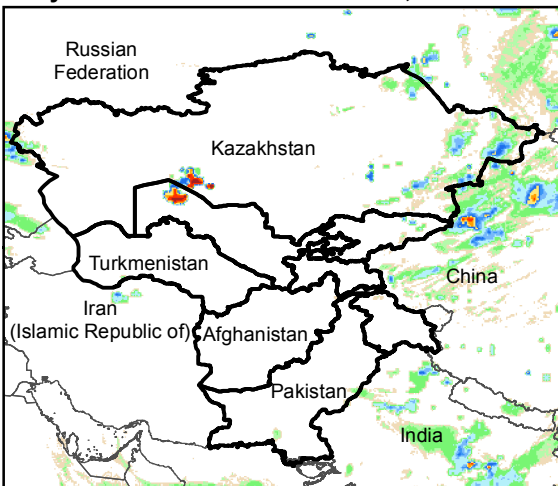
Daily Rainfall estimate for 19 Jun., 2019
