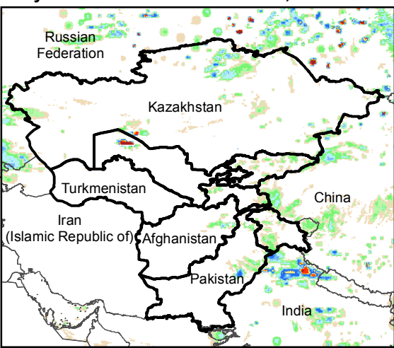
Daily Rainfall estimate for 17 Jun., 2019
