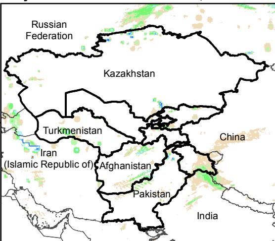
Daily Rainfall estimate for 26 Nov., 2019
