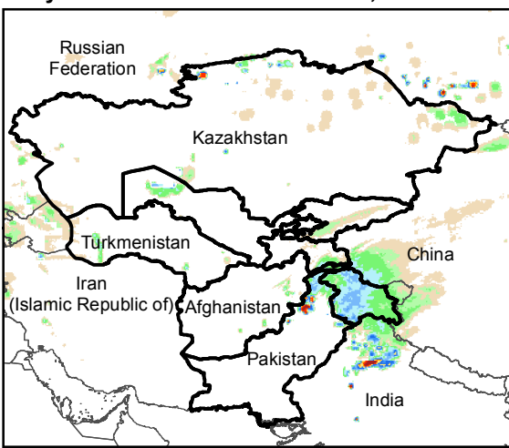
Daily Rainfall estimate for 27 Nov., 2019
