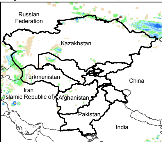
Daily Rainfall estimate for 29 Dec., 2019
