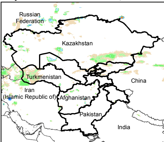
Daily Rainfall estimate for 31 Dec., 2019
