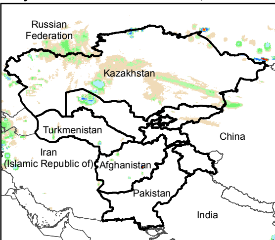
Daily Rainfall estimate for 30 Dec., 2019
