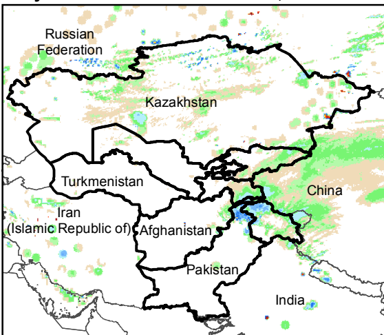
Daily Rainfall estimate for 17 Jan., 2020
