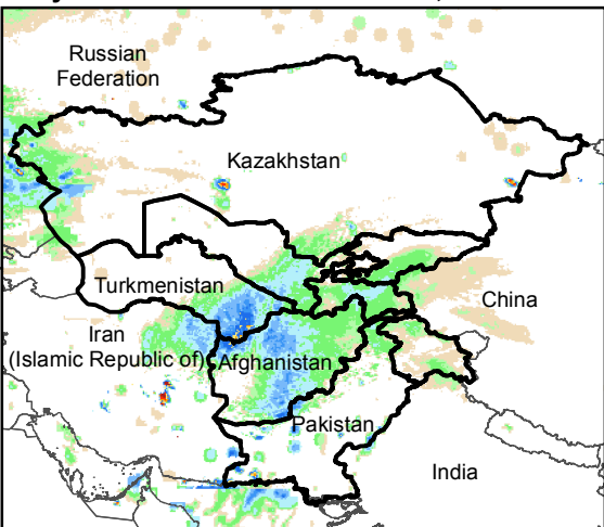
Daily Rainfall estimate for 15 Jan., 2020
