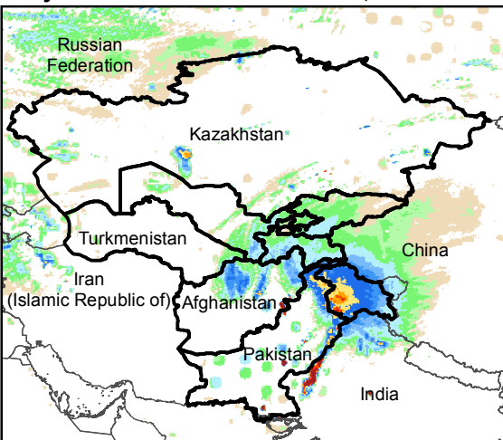
Daily Rainfall estimate for 16 Jan., 2020
