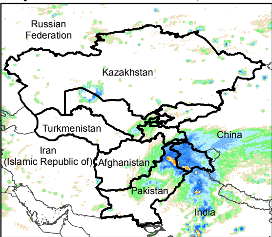
Daily Rainfall estimate for 30 Mar., 2020
