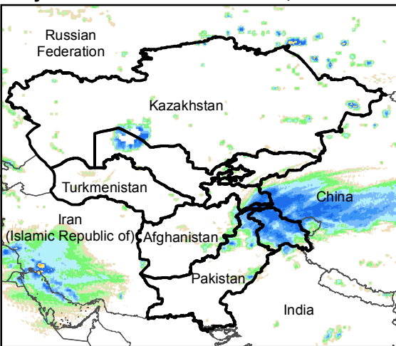
Daily Rainfall estimate for 31 Mar., 2020
