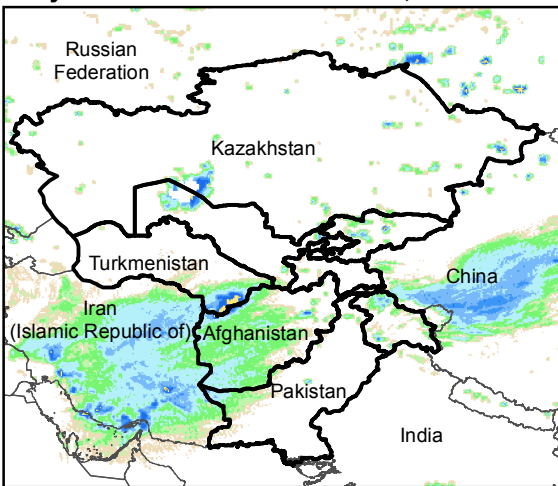
Daily Rainfall estimate for 1 Apr., 2020
