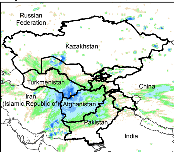
Daily Rainfall estimate for 2 Apr., 2020
