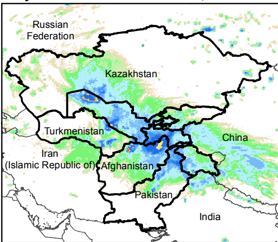
Daily Rainfall estimate for 3 Apr., 2020
